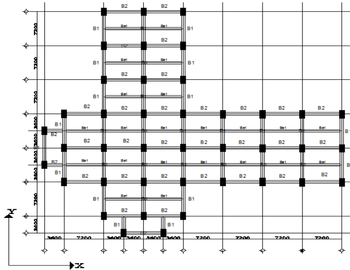
Gambar L-1.3 Denah Balok Model 3
