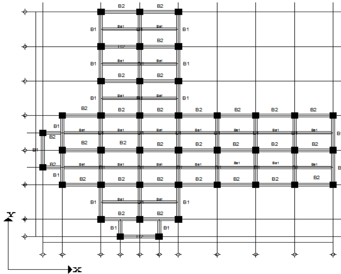
Gambar L-1.1 Denah Balok Model 1
