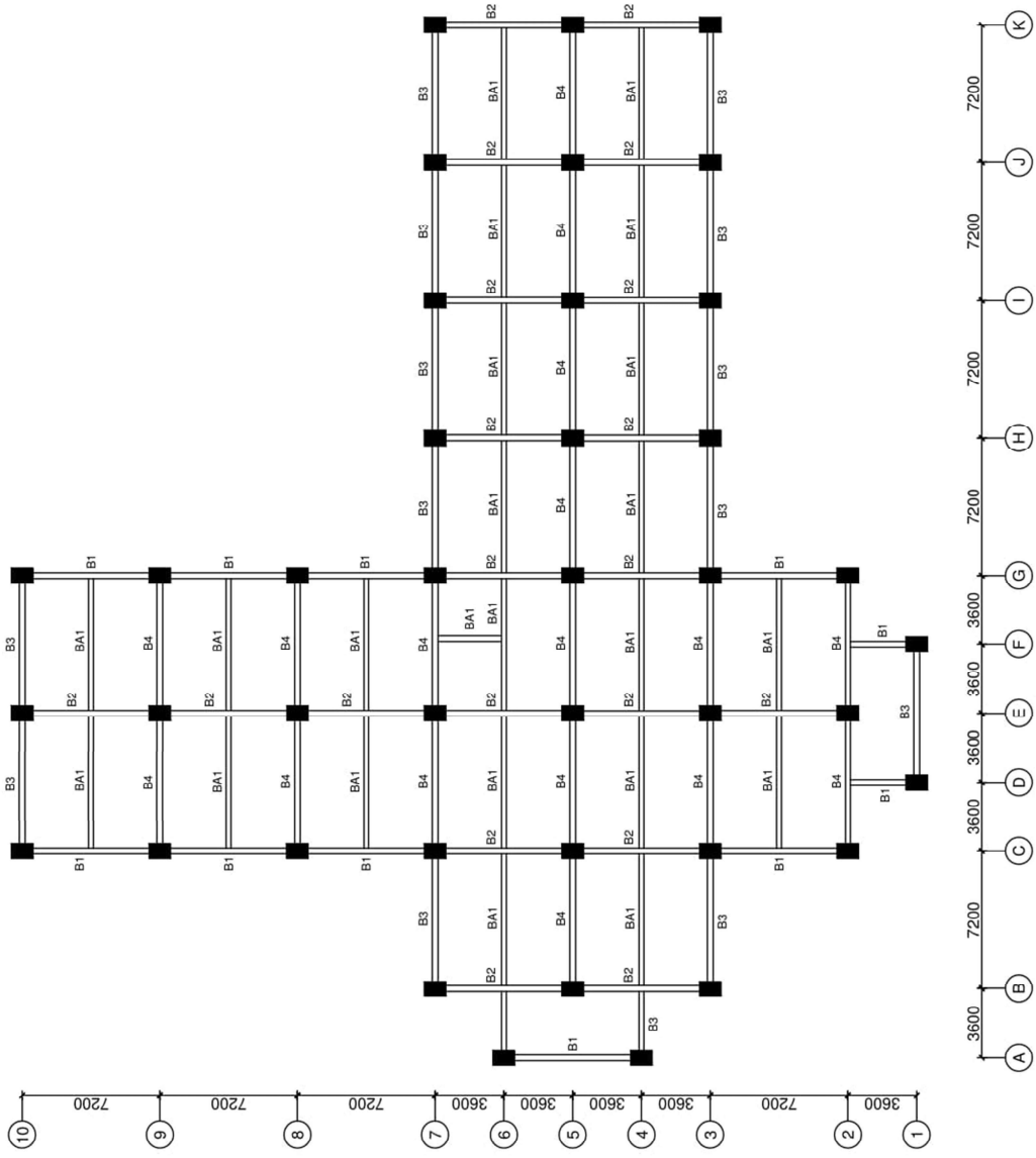
Lampiran 2. Denah Balok Model 2
