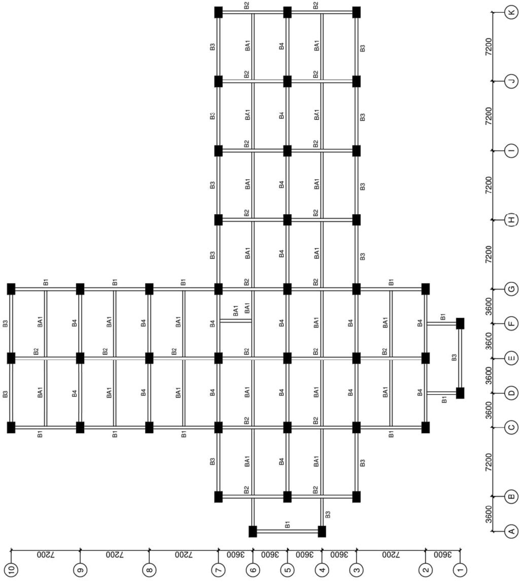
Lampiran 1. Denah Balok Model 1
