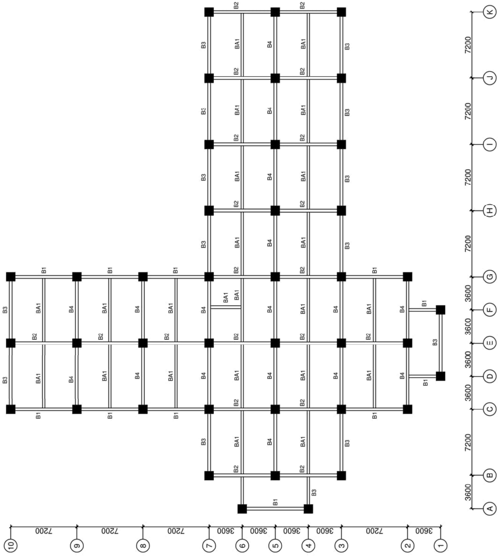
Lampiran 4. Denah Balok Model 4
