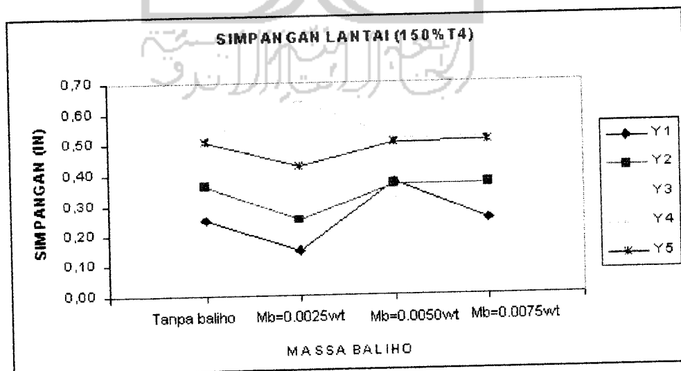
Gambar 5.5a. Simpanan Lantai (150%T4)
