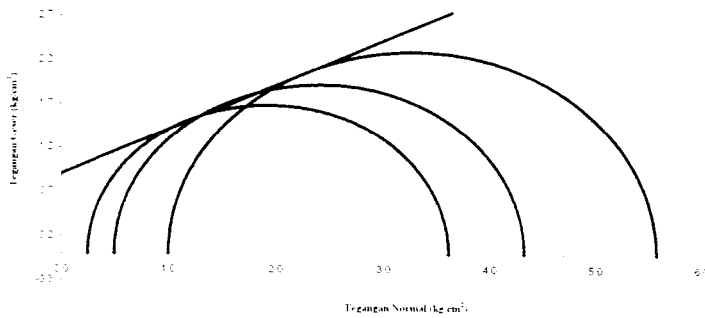
Diagram Mohr
