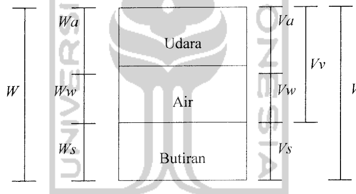
Gambar 3.2 Diagram Fase Tanah (HC Hardiyatmo, 1992)
