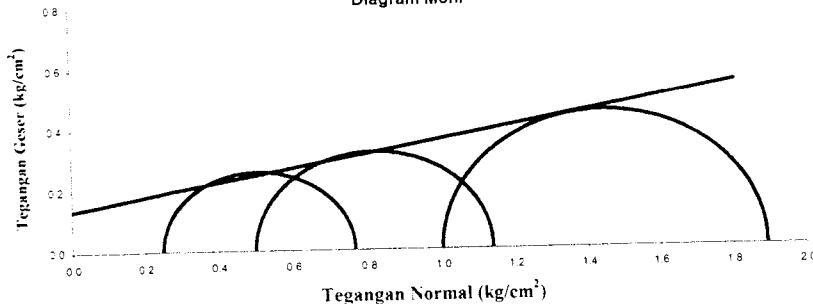
Diagram Mohr
