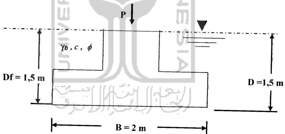
Gambar 5.8 Detail Pondasi
