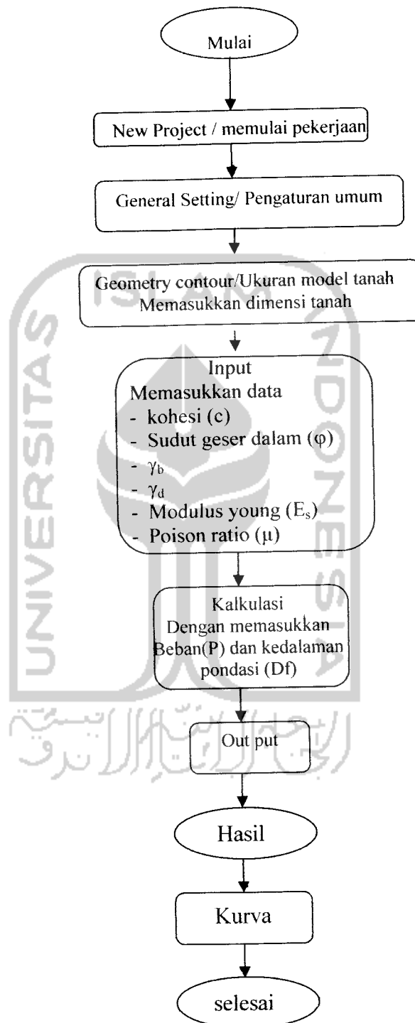
Gambar 4.35 Diagram Alir Program Plaxis
