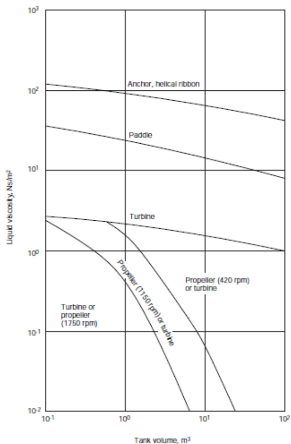
Figure 10.57. Agitator selection guide
