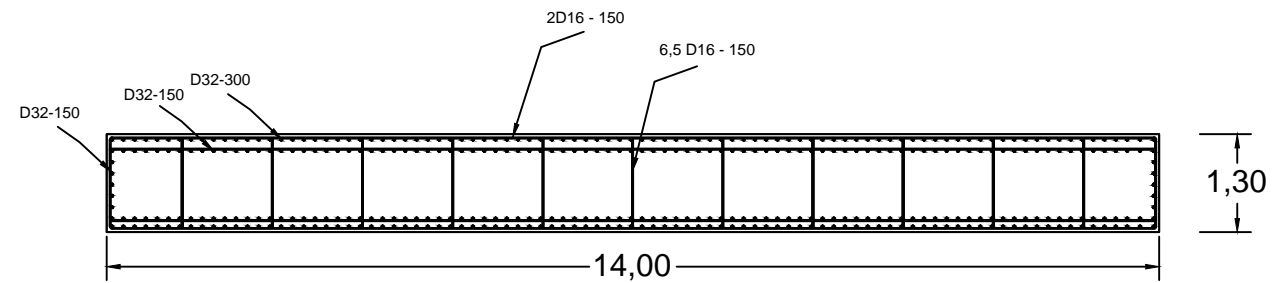
DETAIL PENULANGAN ABUTMEN
