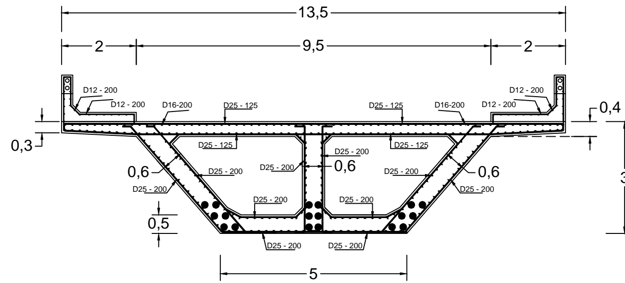
GAMBAR DETAIL PENULANGAN BOX GIRDER
