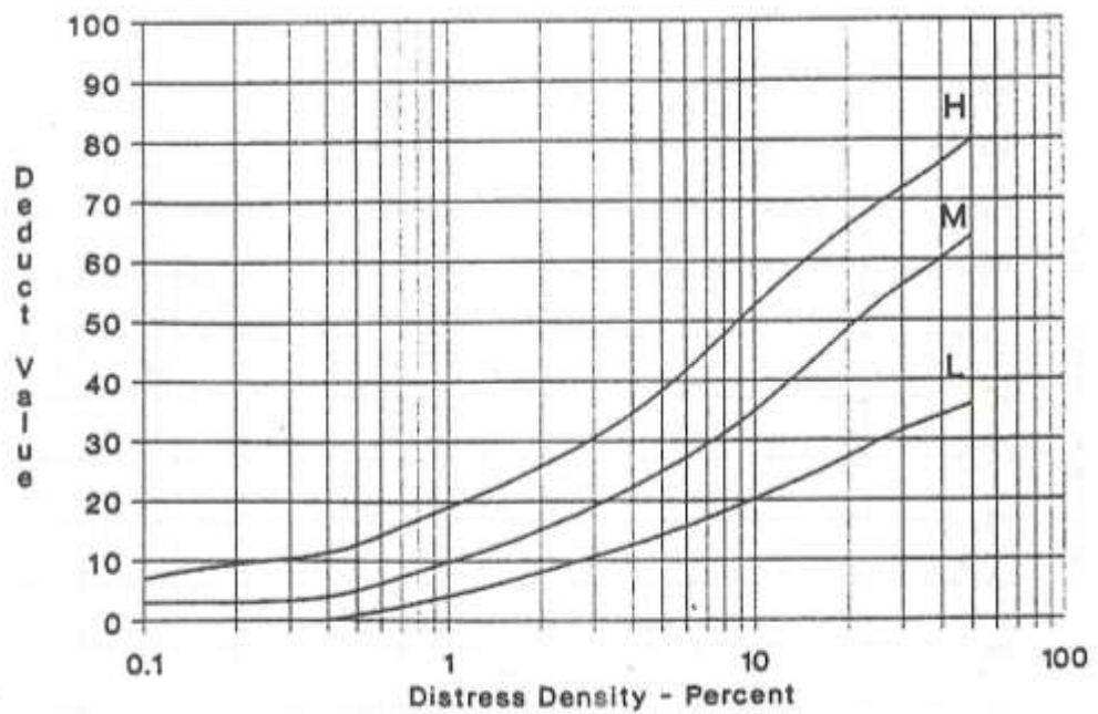
Sungkur ( Shoving )
