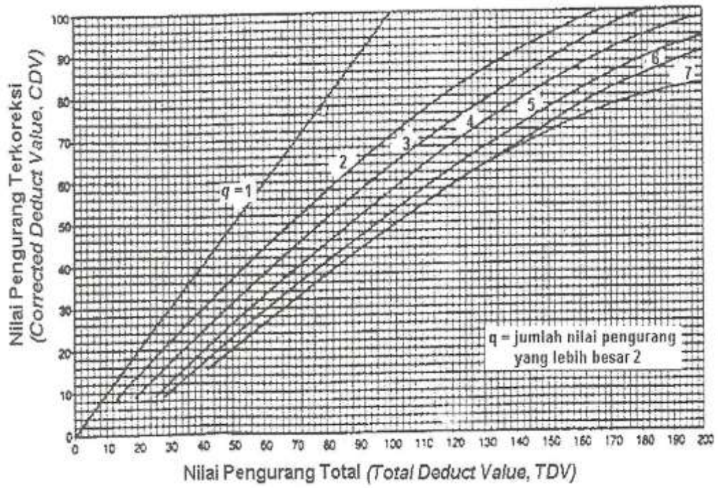
Grafik Corrected Deduct Value (CDV)
