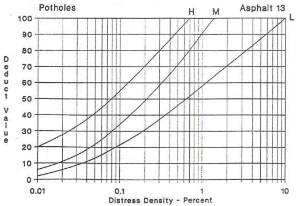
Lubang( Potholes )
