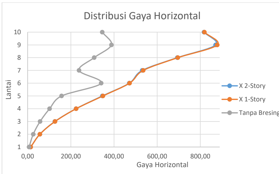
Gambar L-4.2 Distribusi Gaya Horizontal
