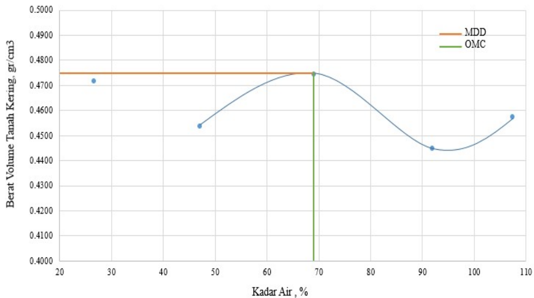
Berat volume kering vs kadar air
