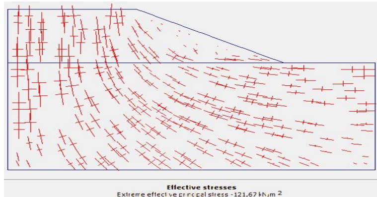
Effective Stresses
