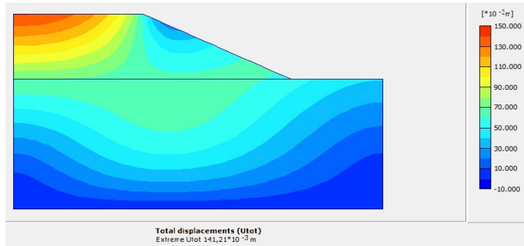
Total Displacement (0.138m)
