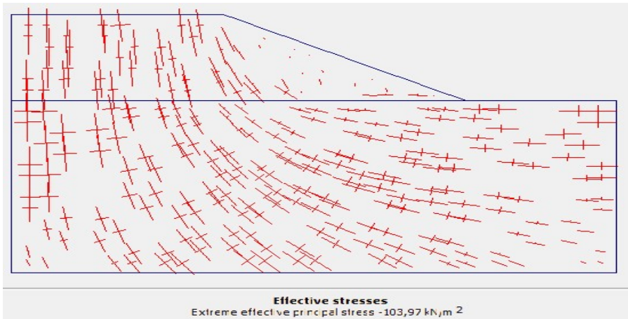
Effective Stresses
