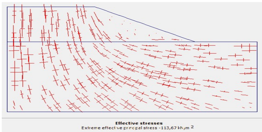
Effective Stresses
