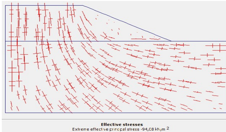
Effective Stresses
