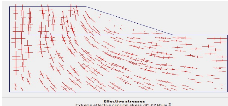
Effective Stresses
