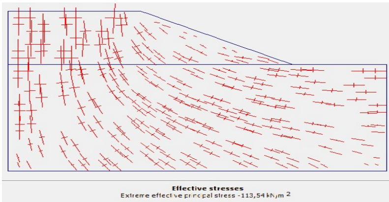
Effective Stresses
