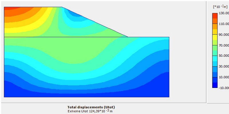
Total Displacement (0,124m)
