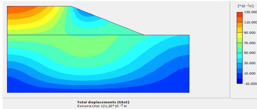
Total Displacement (0.121m)
