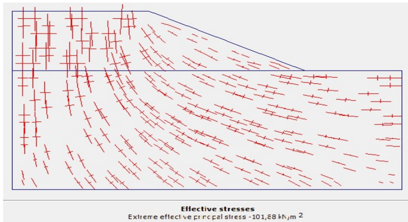
Effective Stresses
