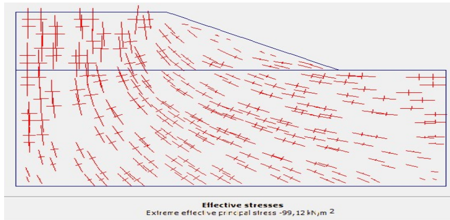
Effective Stresses
