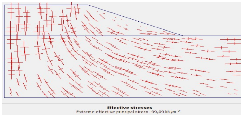
Effective Stresses
