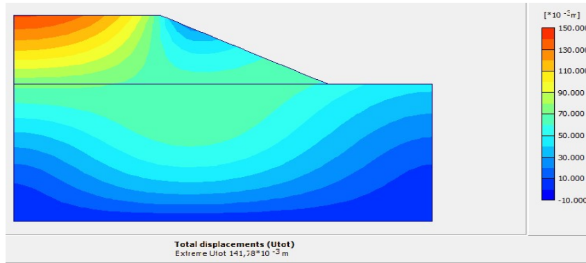
Total Displacement (0,142m)
