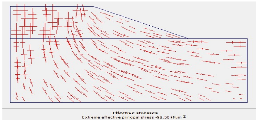
Effective Stresses
