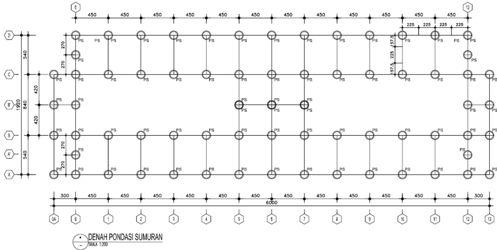
Lampiran 1 Denah Pondasi Sumuran
