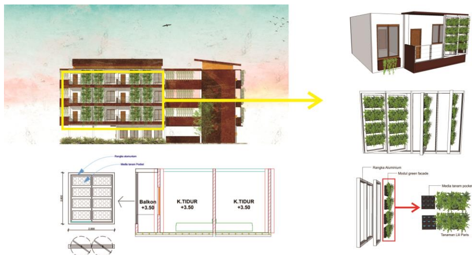
Gambar 5. 5 Detail green facade 1
