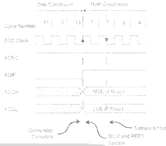
Figure 94. ADC Timing Diagram, Free Running Conversion
