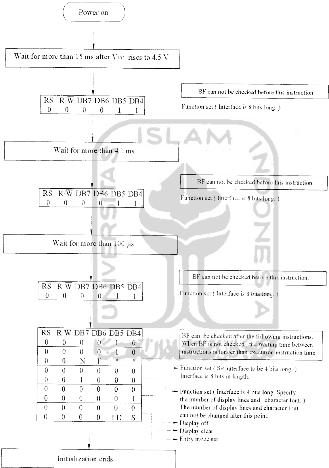
4-Bit Ineterface
