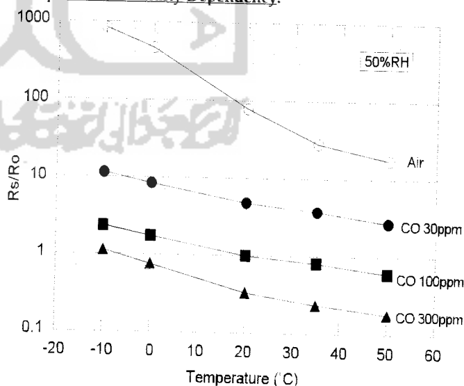
Temperature/Humidity Dependency:
