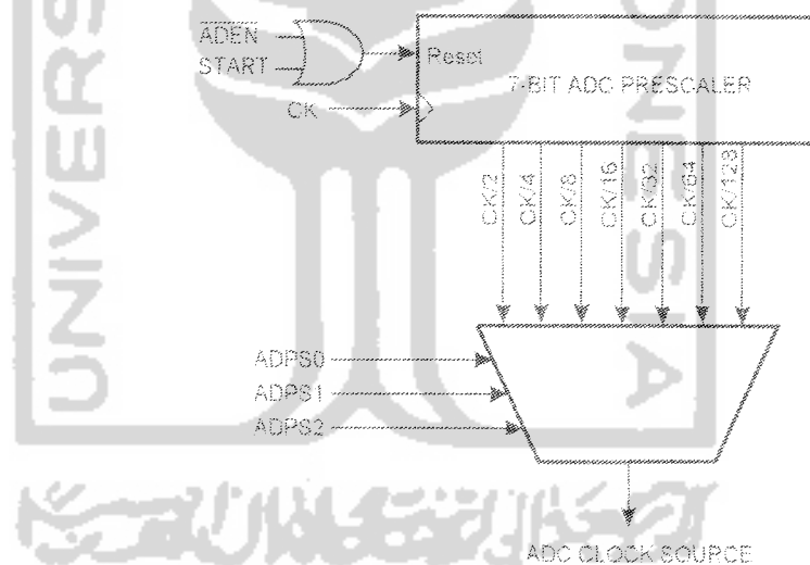
Figure 91. ADC Prescaler
