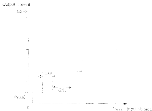
Figure 100. Differential Non-linearity (DNL)
