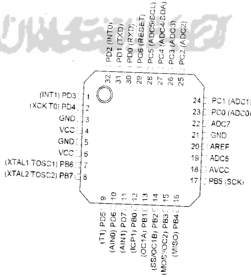
MLF Top View
