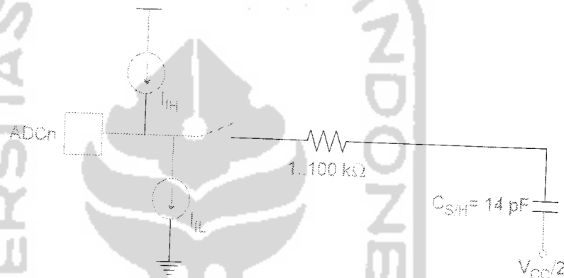
Figure 95. Analog Input Circuitry
