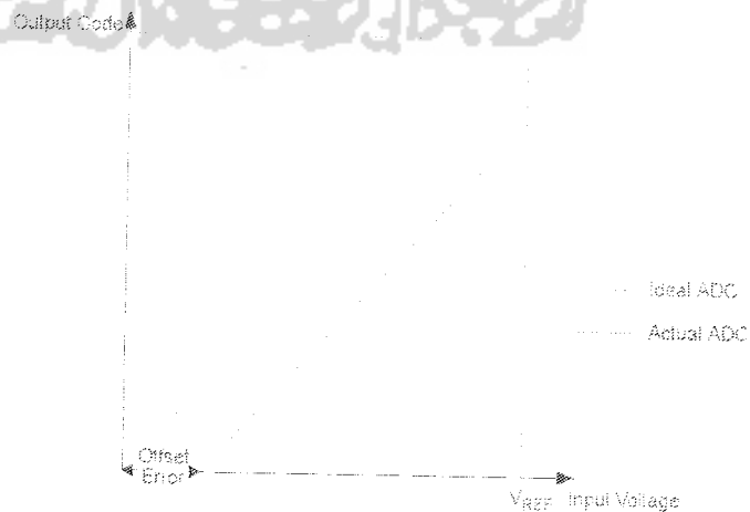
Figure 97. Offset Error
