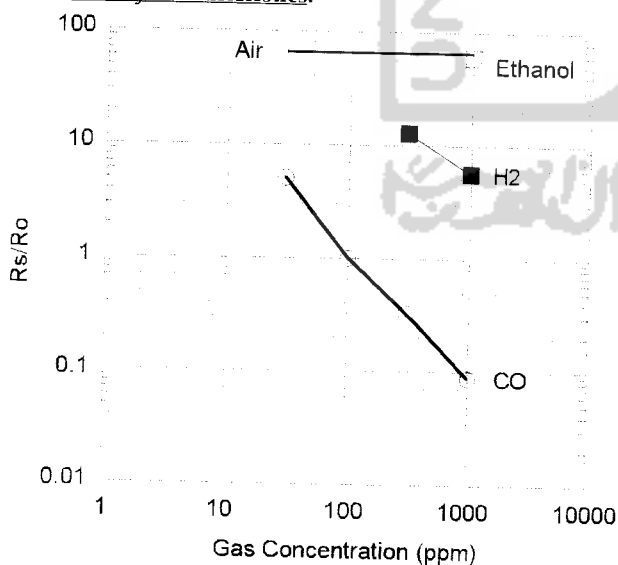
Sensitivity Characteristics:
