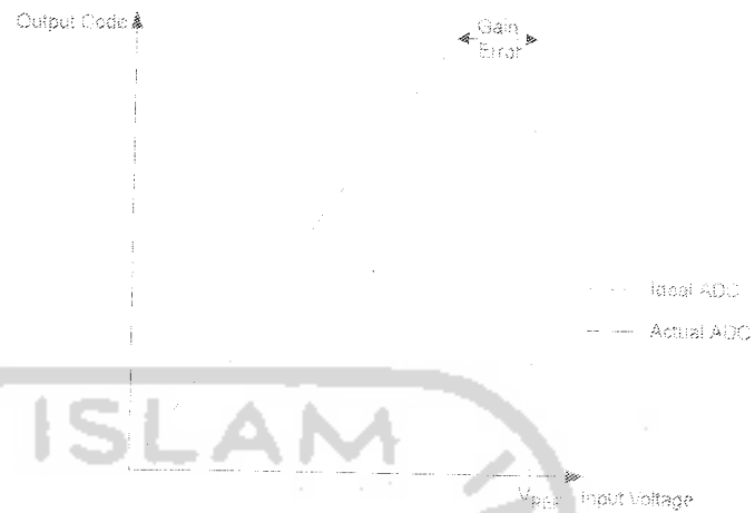
Figure 98. Gain Error
