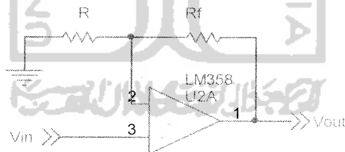
Gambar 2.6. Rangkaian penguat non-inverting
