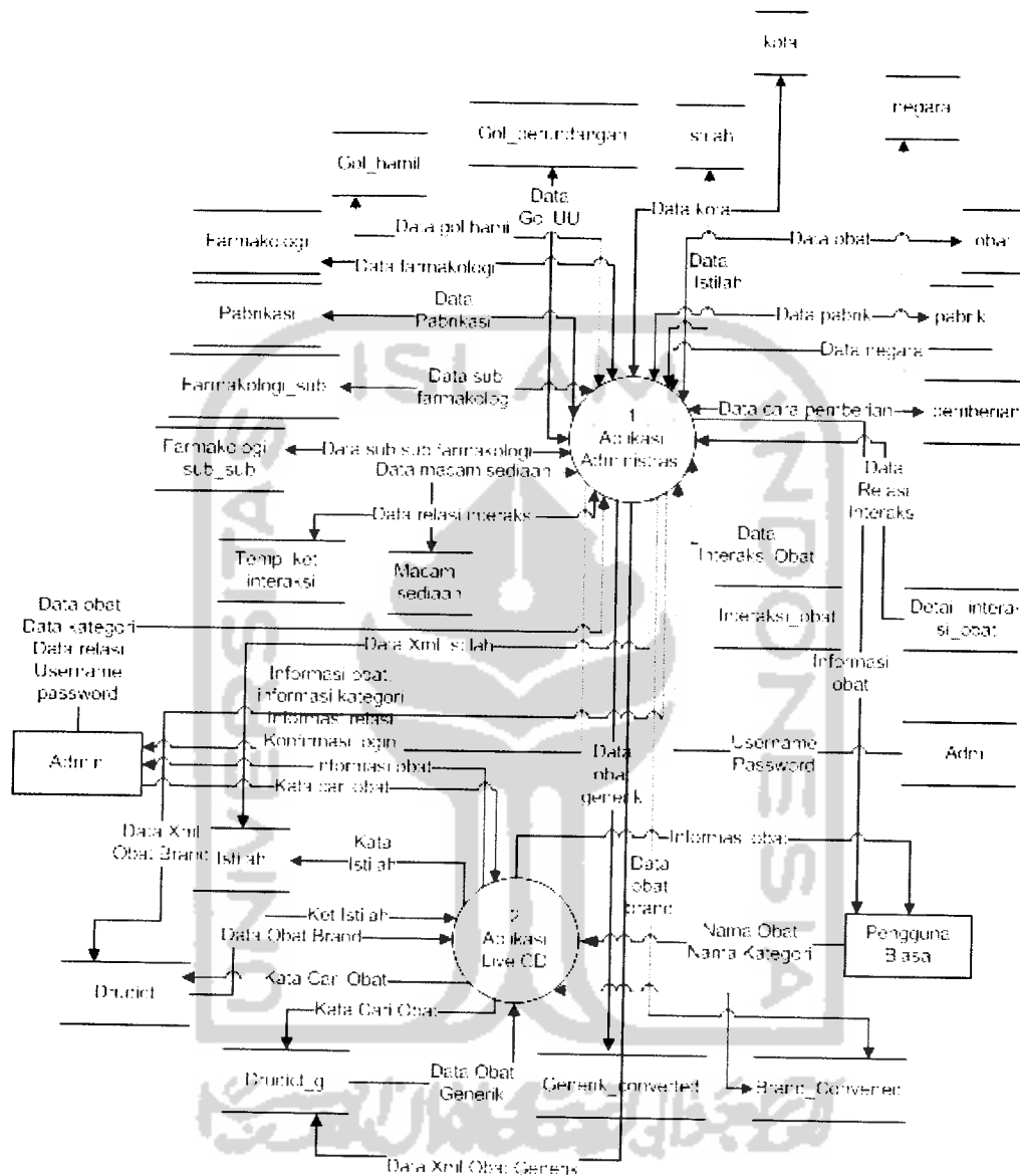
Gambar 3.2. DFD Level 1
