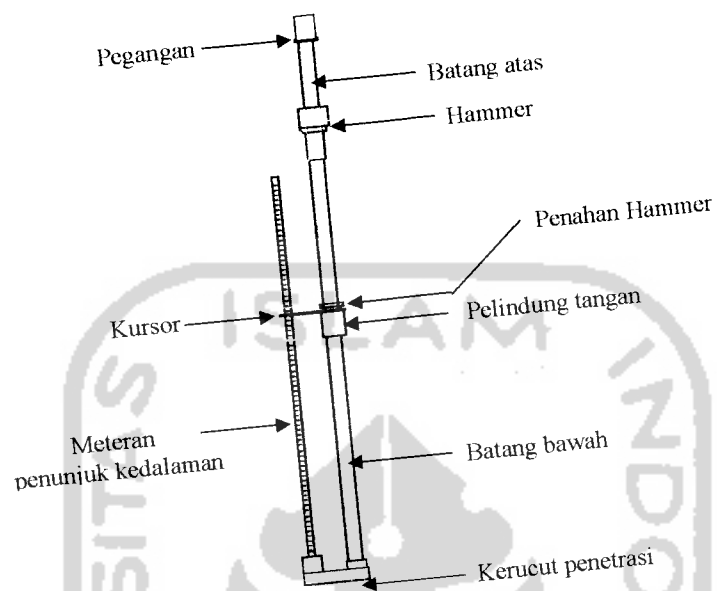
Gambar 3.4 Alat Dinamic Cone Penetrometer (DCP) Sumber : Manual DCP
