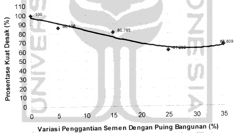
Gambar 6.12 Grafik nilai prosentase kuat desak paving block
